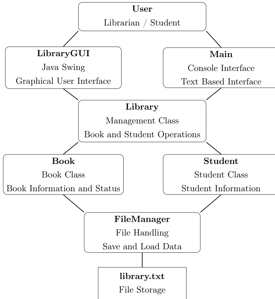
Figure 3.1: System Architecture of Library Management System
